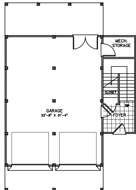
GARAGE FLOOR PLAN
